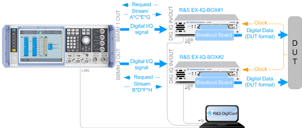
Figure 5-1: Simplified test setup for 2x8 MIMO tests with "slow IQ" signals
