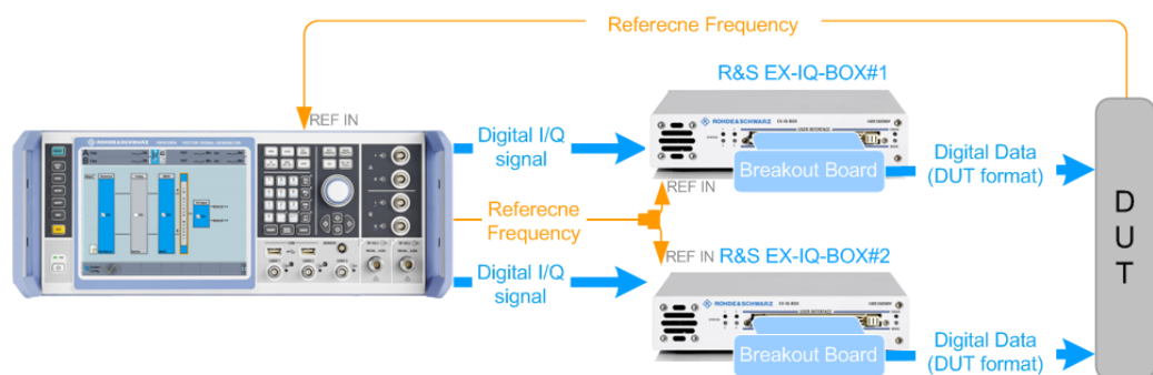
Figure 3-4: Simplified test setup for MIMO tests with external reference signal
