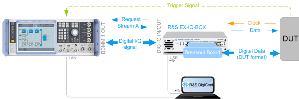
Figure 3-1: Simplified test setup for SISO tests with "slow IQ" signals
